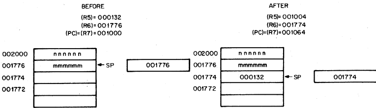
Figure 5-8: JSR
