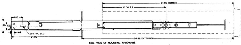
Figure 6-6 Side View of Mounting Hardware
