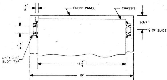
Figure 6-5 Rear View of Mounting Hardware
